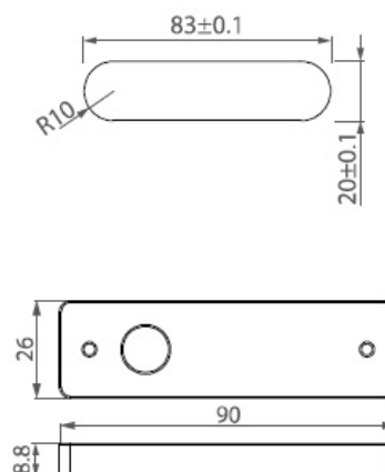
drilling template
